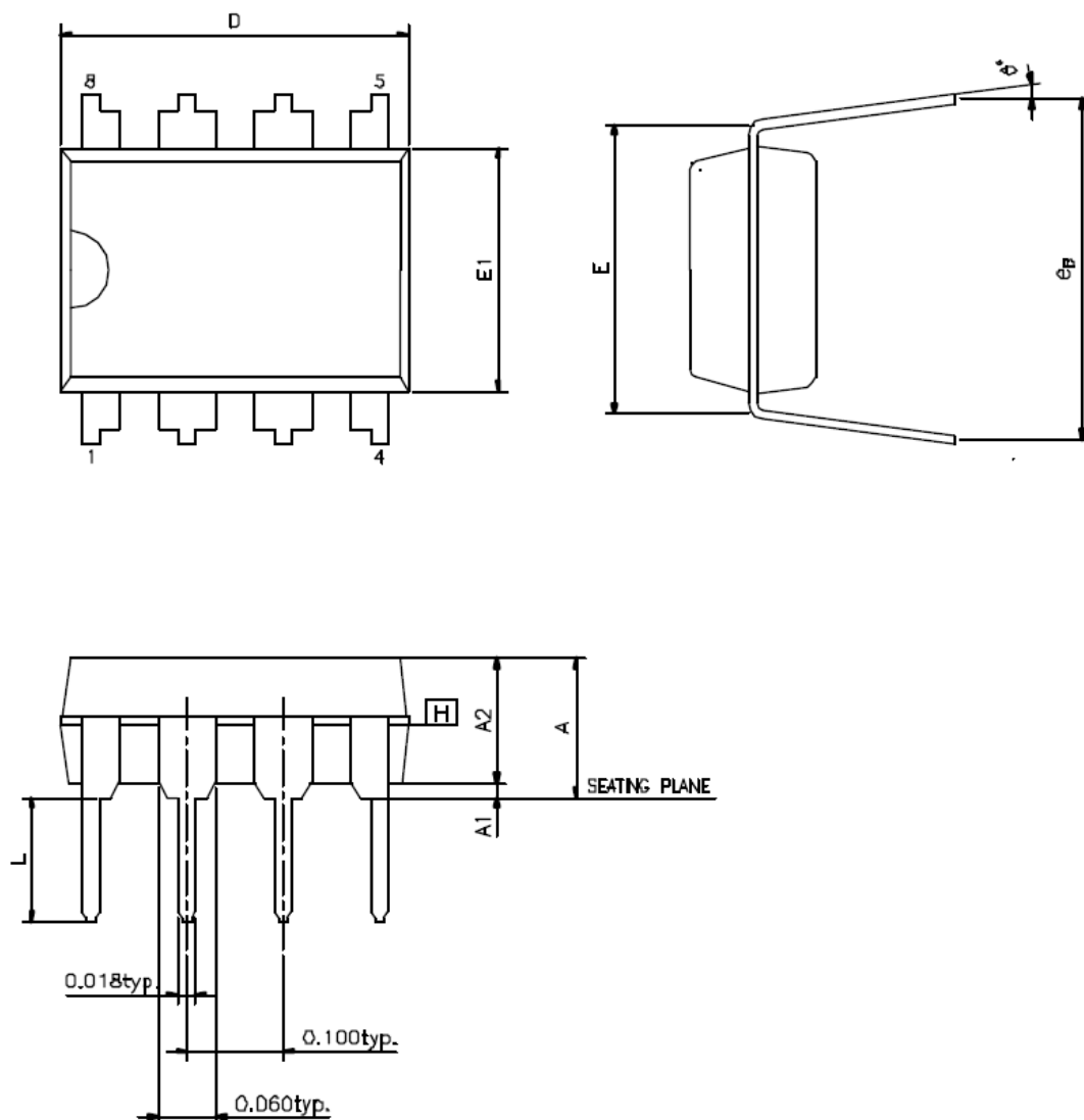
Figure 33. PDIP8
