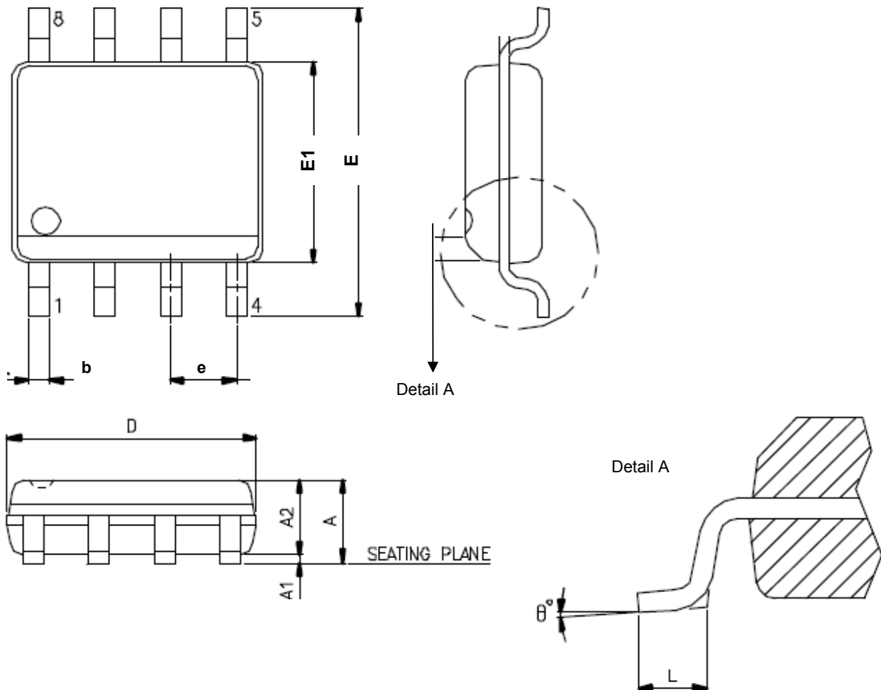
Figure 30. SOP 8 ( 150 mil )
