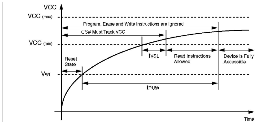
Figure 26. Power-up Timing
