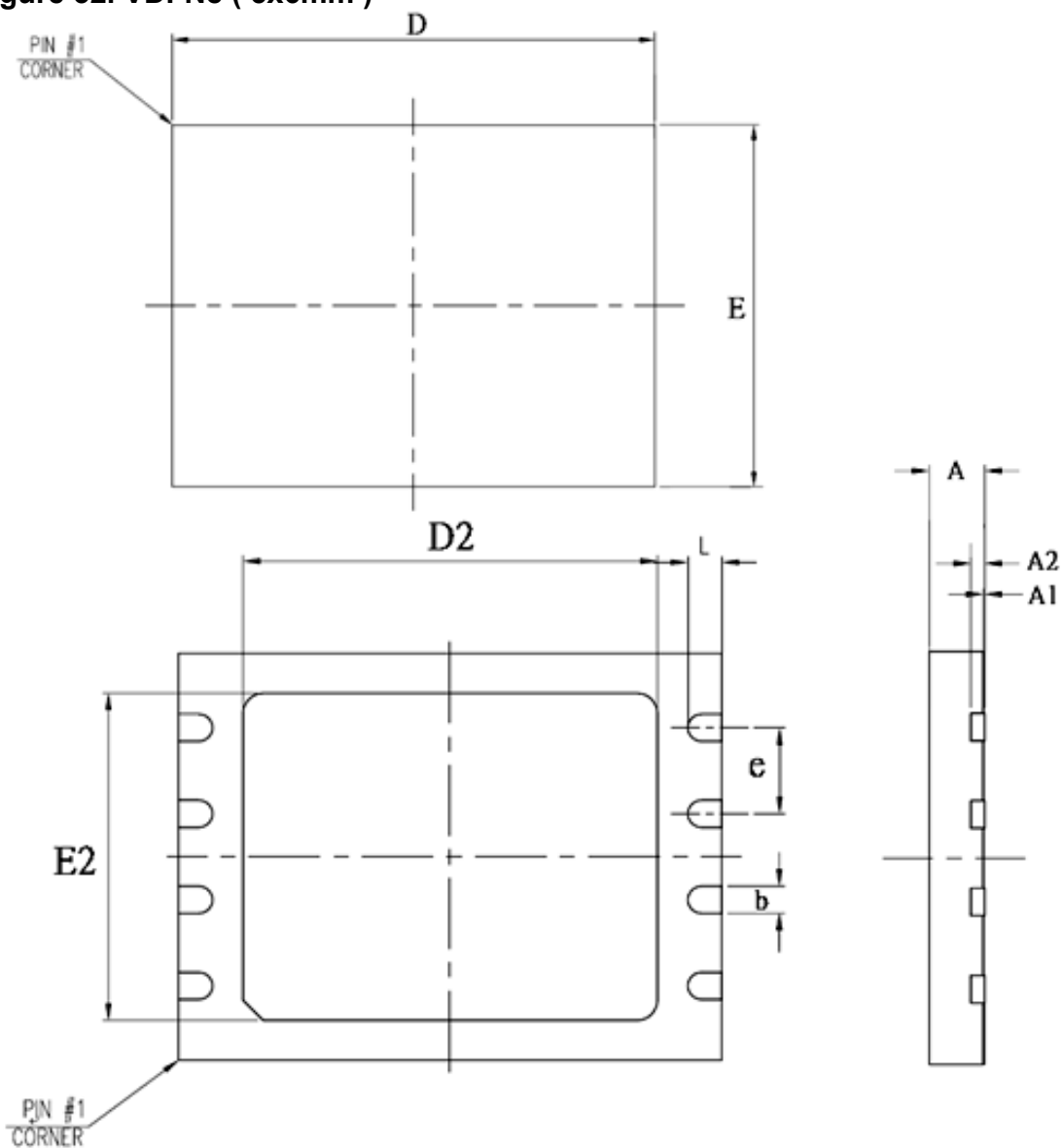
Figure 32. VDFN8 ( 5x6mm )
