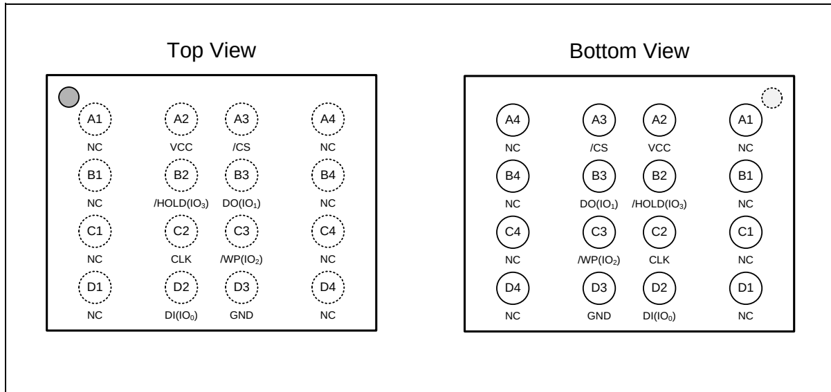
Figure 1e. W25Q64FW Ball Assignments, 16-ball WLPGA (Package Code BY)
